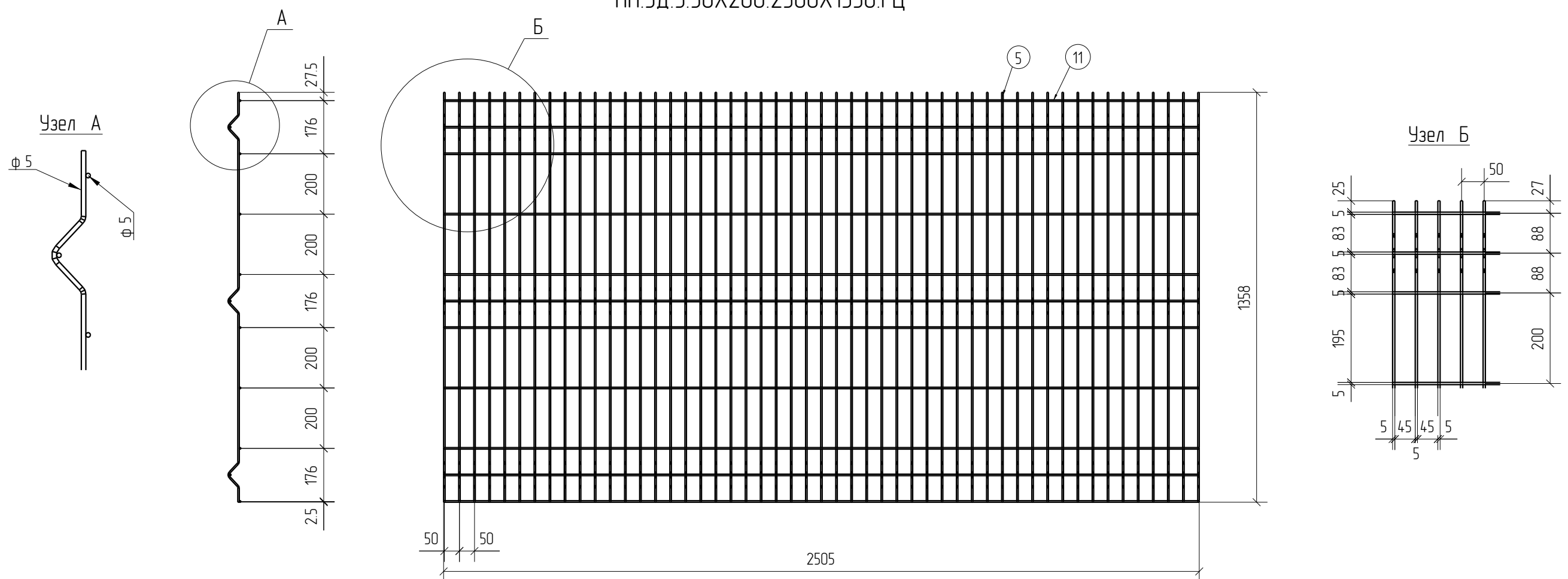
ПН.ЗД.5.50X200.2500X1358.ГЦ
