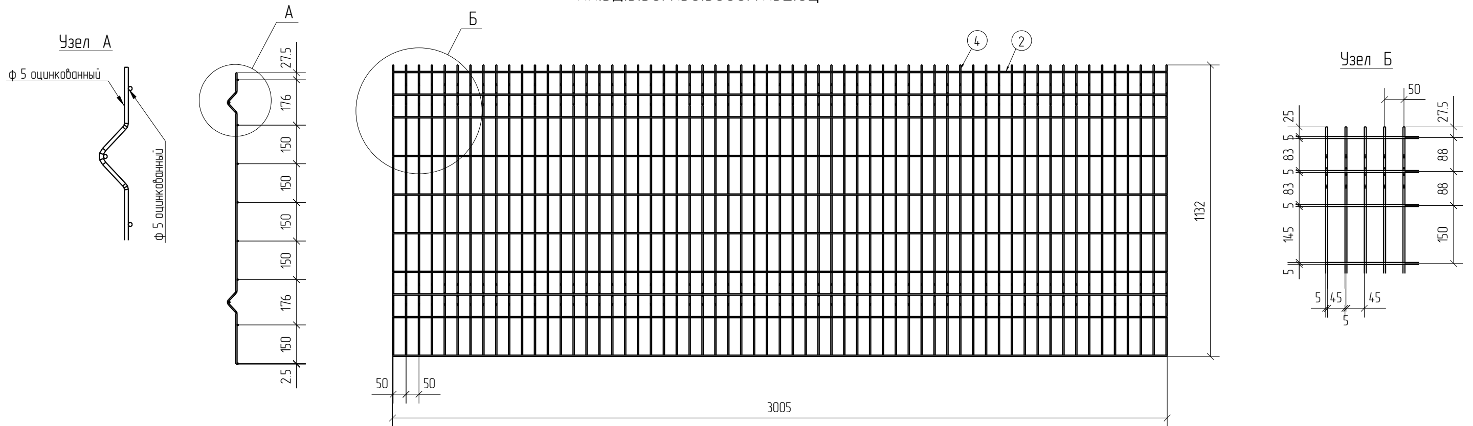
ПН.ЗД.5.50X150.3000X1132.0Ц
