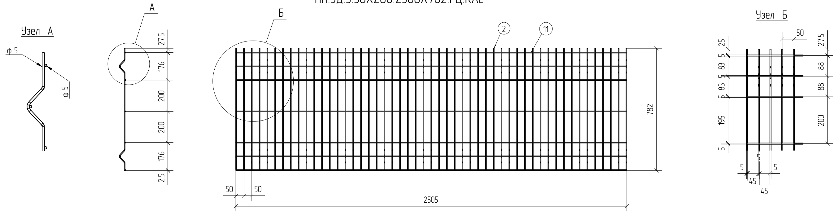
ПН.ЗД.5.50X200.2500X782.ГЦ.RAL
